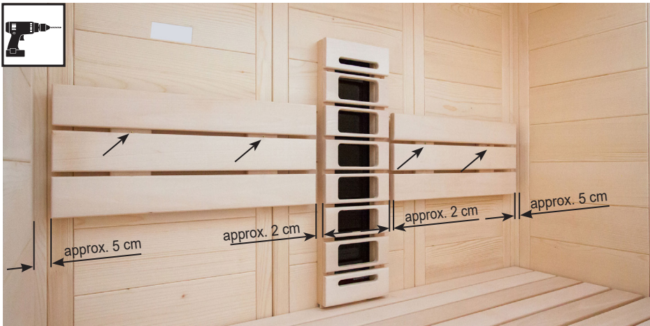
3 mm drill bit, 4 screws 4 x 70 mm
