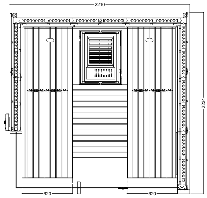
assembly right
